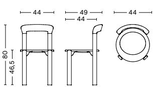
REY CHAIR WIDTH 44 CM DEPTH 49 CM HEIGHT 80 CM SEAT HEIGHT 46,5 CM SEAT DEPTH 44 CM
