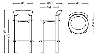
REY BAR STOOL WIDTH 45 CM DEPTH 49,5 CM HEIGHT 97 CM SEAT HEIGHT 75 CM SEAT DEPTH 44 CM
