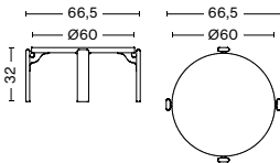
REY COFFEE TABLE WIDTH 66,5 CM LENGTH 66,5 CM HEIGHT 32 CM DIAMETER TABLETOP 60 CM
