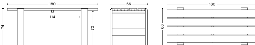
WEEKDAY TABLE 180 LENGTH 180 CM WIDTH 66 CM HEIGHT 74 CM
